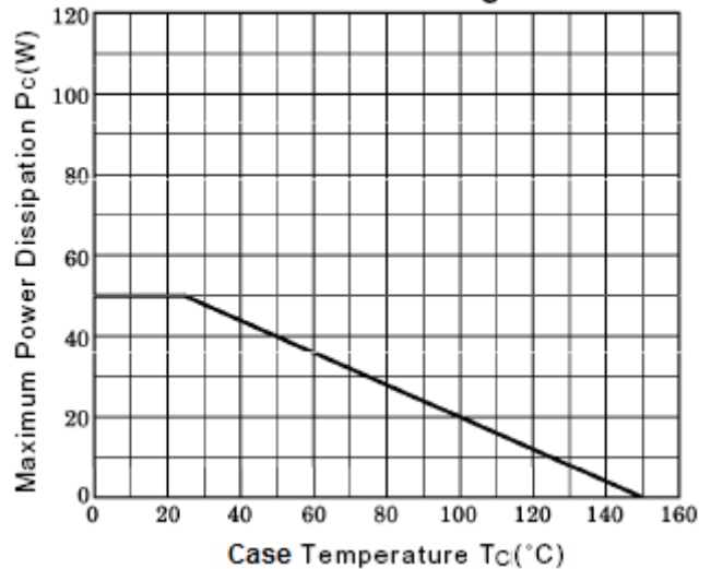
Power Derating
